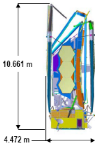
Stowed Configuration
